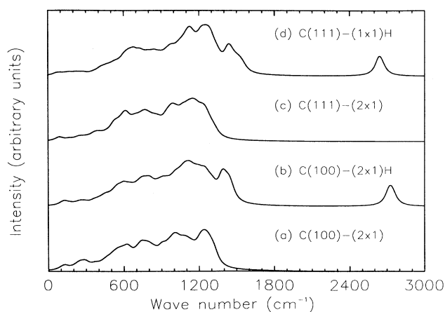
FIG. 1. Projected vibrational density of states of the diamond (100) and (111) surfaces; (a) clean (100)-(2×1), (b) hydrogenated (100)-(2×1), (c) clean (111)-(2×1), and (d) hydrogenated (111) surfaces.
